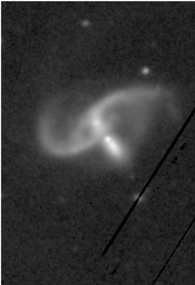
I, CTIO 15m 19 Nov 1992
