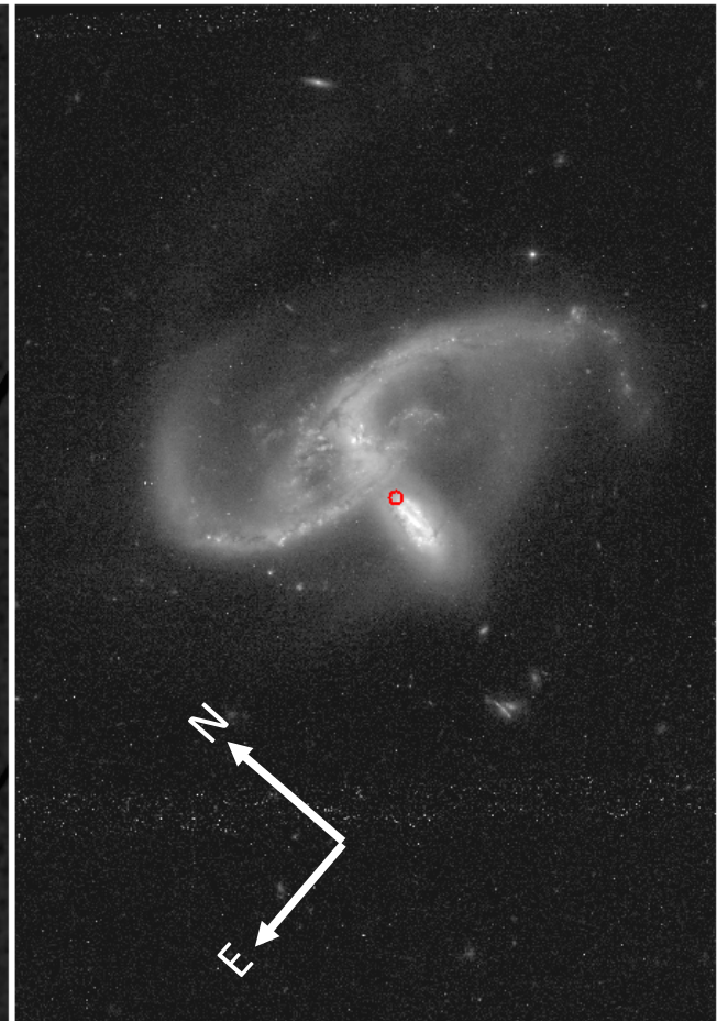
ACS F606W HST 21 Sept 2019
