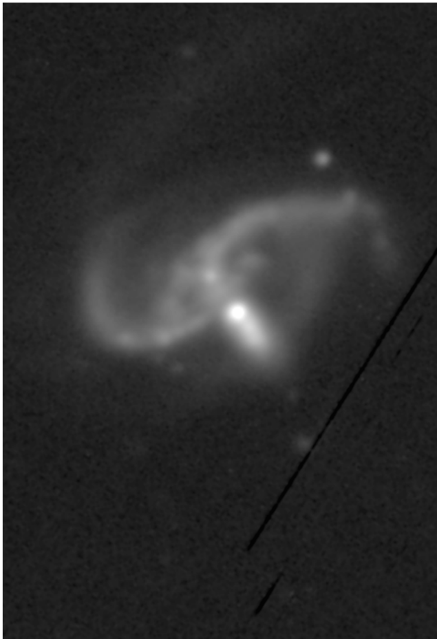
B, CTIO 1.5m 19 Nov 1992
