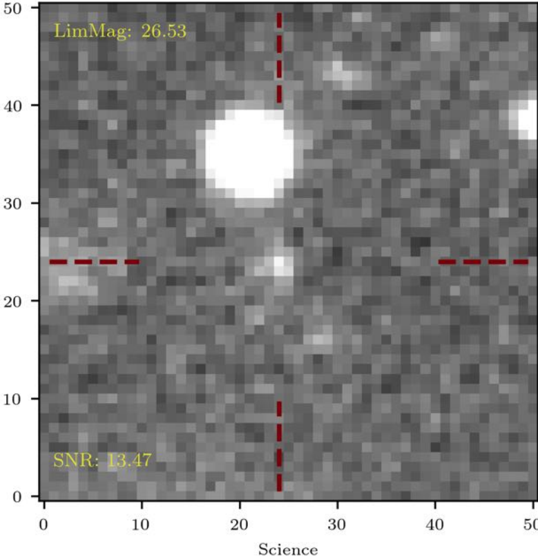
Sloan-i 24.81 [0.081] mag
