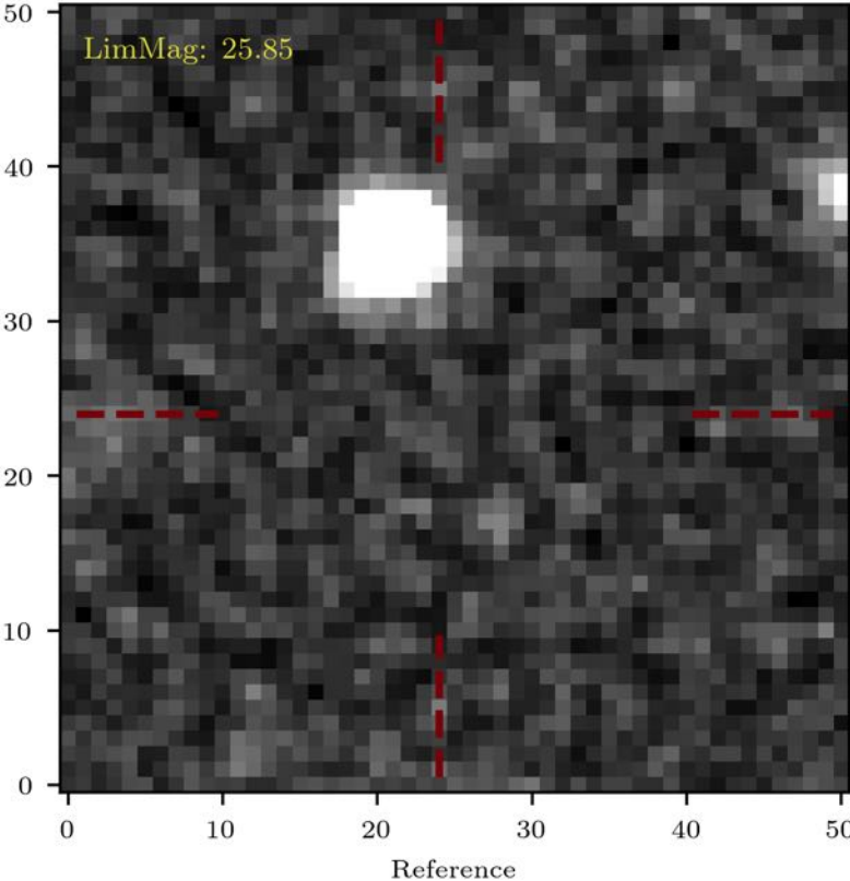
NonDetection 21:06:41.614 -65:55:42.85
