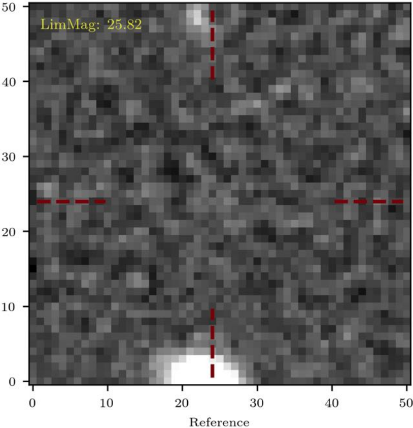
NonDetection 21:04:24.515 -66:45:47.38
