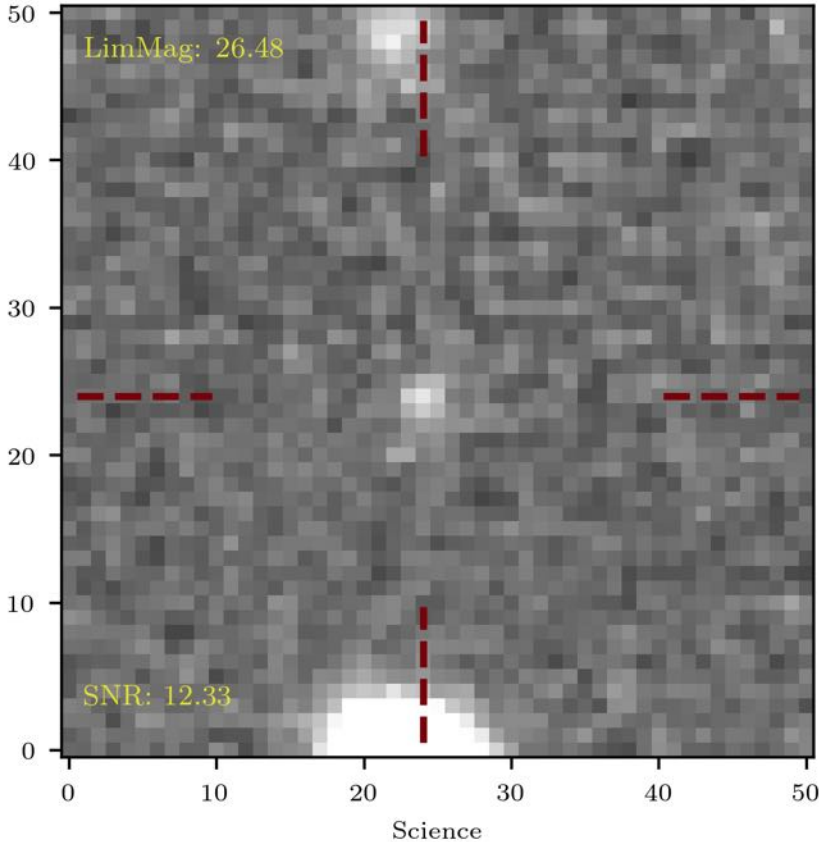
Sloan-i 24.86 [0.088] mag
