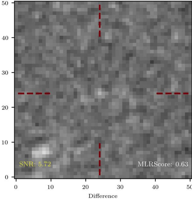
Sloan-i 25.73 [0.190] mag
