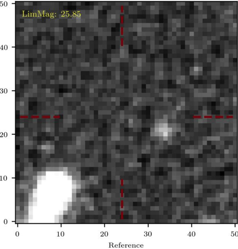
NonDetection 21:02:41.229 -65:46:56.16
