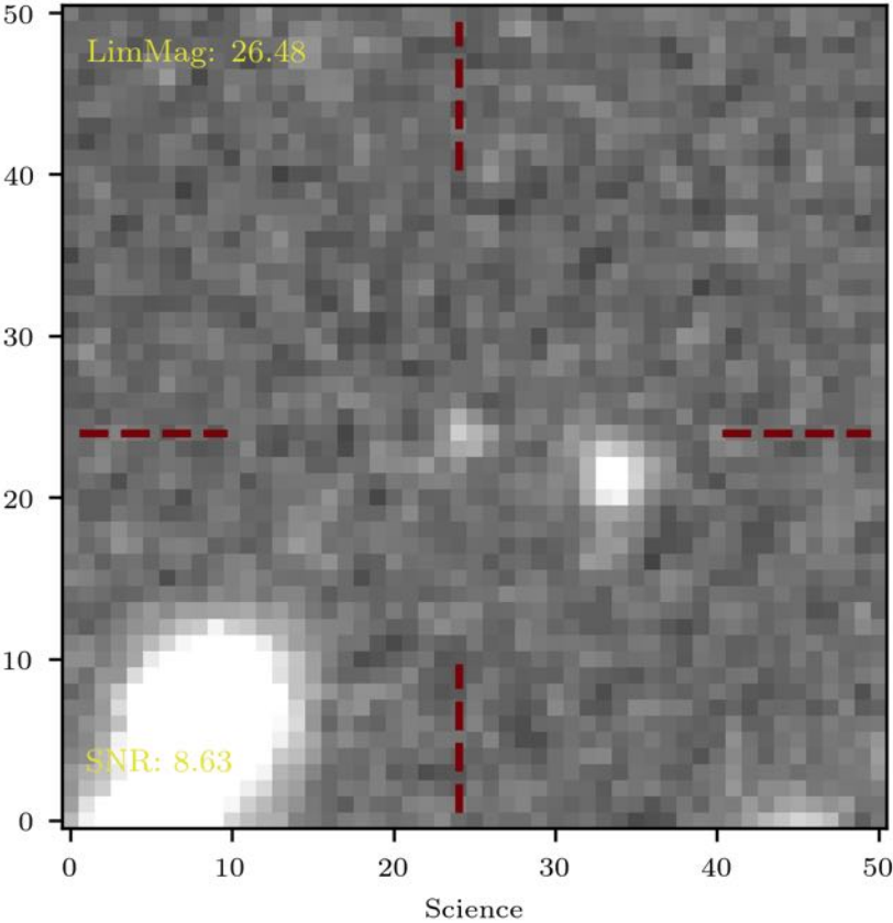
Sloan-i 25.28 [0.126] mag
