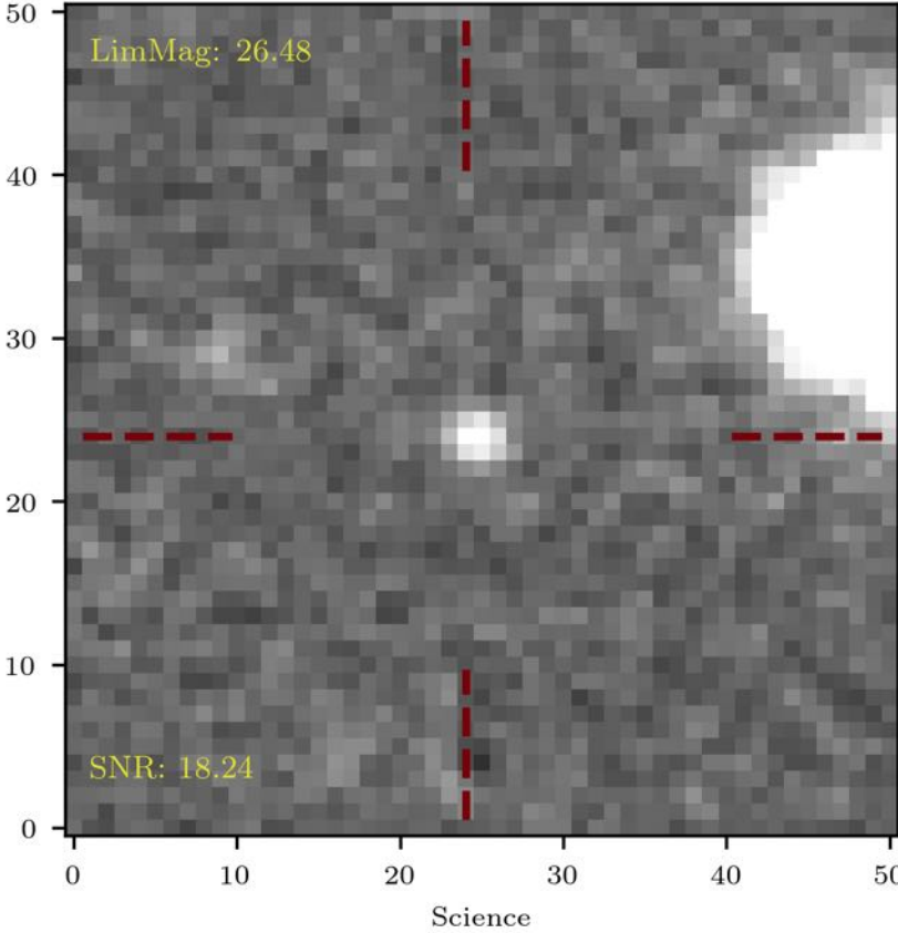
Sloan-i 24.43 [0.060] mag
