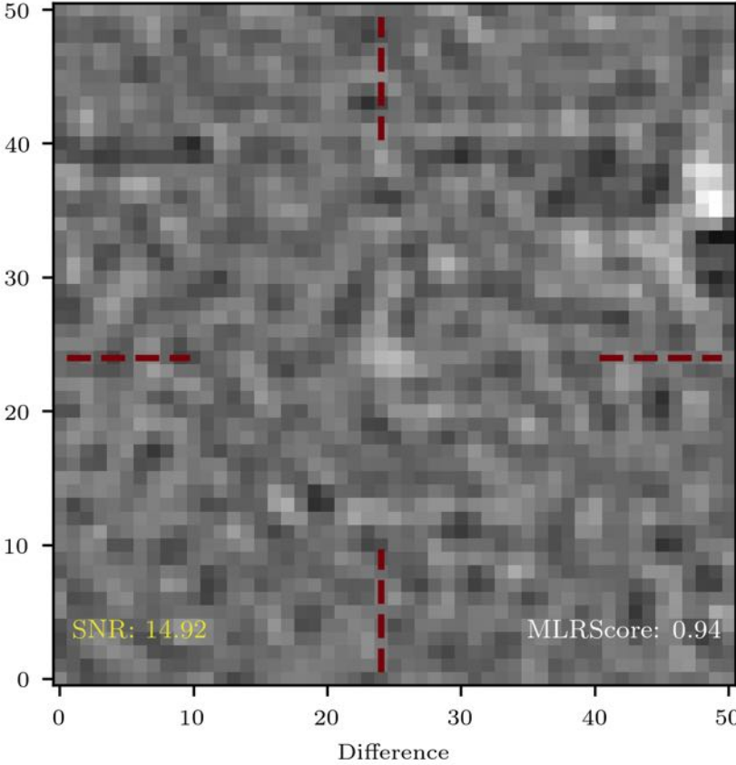
Sloan-i 24.64 [0.073] mag
