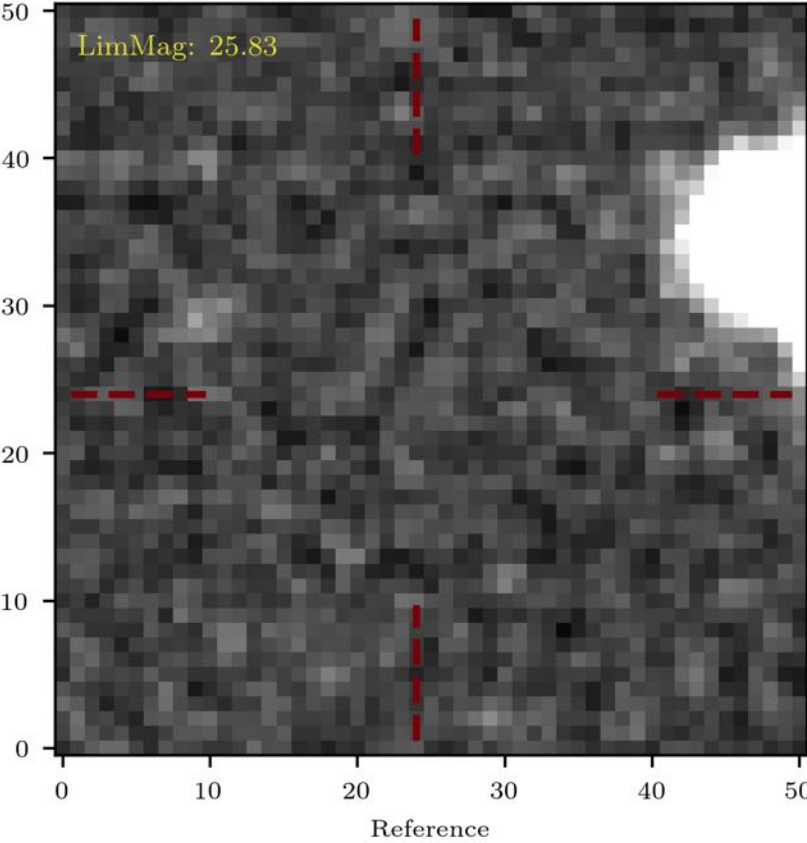
NonDetection 21:12:12.537 -65:27:02.06
